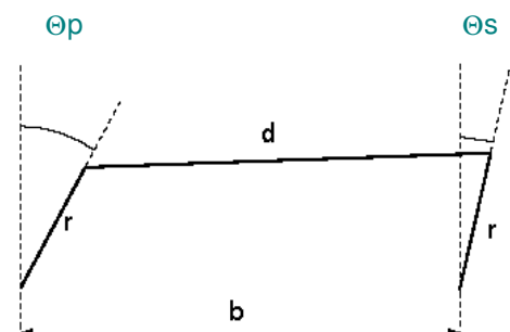
Fig. 2 Tiller geometry.
